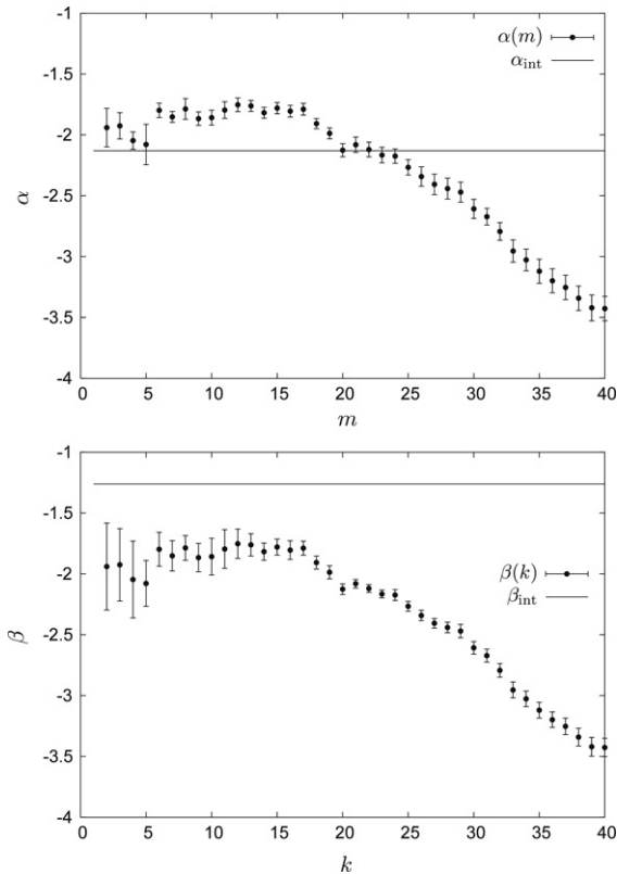
Fig. 7. Power-law exponents of Run III. See the caption of Fig. 6 for details.
