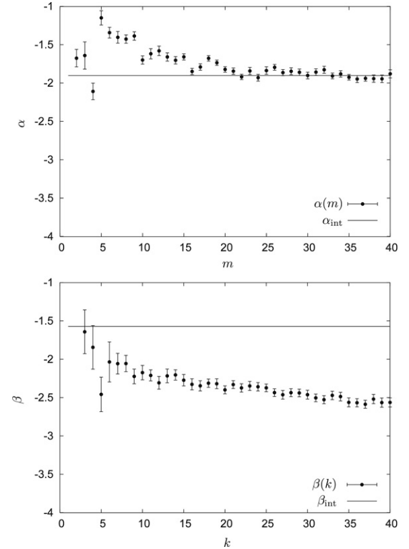
Fig. 6. Power-law exponents of each cross-sectional spectrum in Run II. top: \alpha(|m|) , which are the exponents of the cross-sectional energy spectra E_m(k) , bottom: \beta(k) , which are the exponents of the cross-sectional energy spectra E_k(|m|) . The error bars are obtained by fitting errors due to the least-squares method. The exponents of the integrated spectra are also shown.
