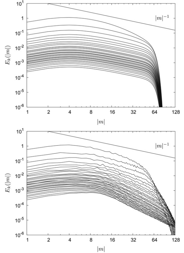
Fig. 1. Cross-sectional spectra E_k(|m|) of GM spectrum as the initial condition (top) and of energy spectrum after about 35 h (bottom) of Run I. Significant differences in the region 16 < |m| < 64 indicates that GM spectrum is not statistically steady.
