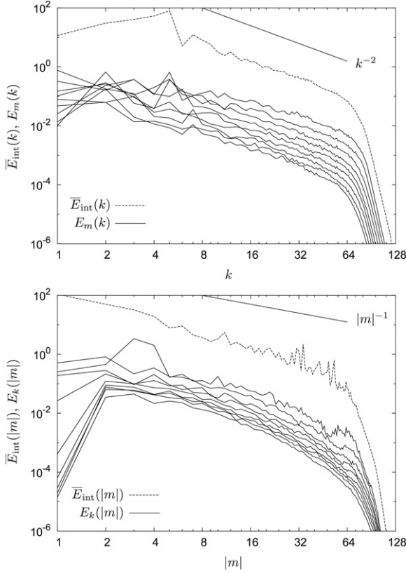
Fig. 4. Integrated energy spectra \bar{E}_{\text{int}}(k) and \bar{E}_{\text{int}}(|m|) , and cross-sectional energy spectra E_m(k) and E_k(|m|) of Run II. The GM spectrum scales as k^{-2}|m|^{-1} for large horizontal and density wavenumbers. The cross-sectional spectra are shown every four curves for visibility.
