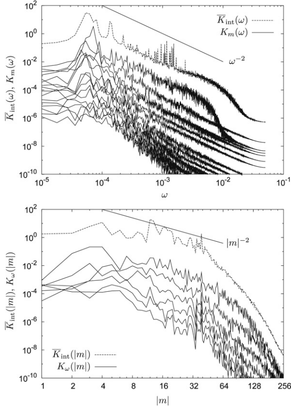
Fig. 11. Integrated kinetic energy spectra, and cross-sectional energy spectra of Run V. The cross-sectional spectra that are functions of frequencies (top) are shown every eight curves for visibility. The cross-sectional spectra that are functions of vertical wavenumbers (bottom) are shown when \omega = 2.5, 5, 10, 20, 40 \times 10^{-4} rad/s. See the caption of Fig. 2 for details.
