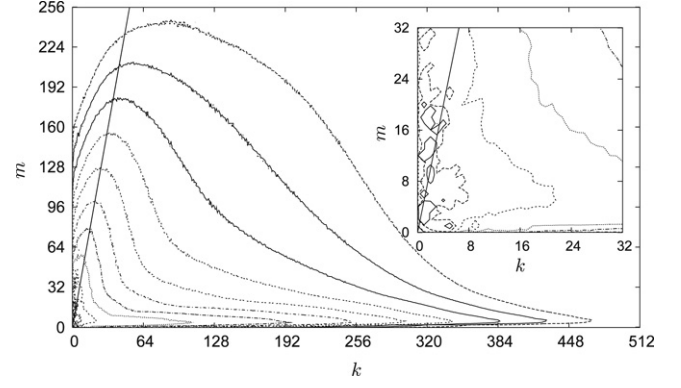
Fig. 9. Two-dimensional energy spectrum E(k, |m|) of Run V. The contours are plotted every powers of ten from 10^{-10} to 1. The straight line from the origin shows the wavenumbers \omega = 1.5f . The inset is the enlargement of the area near the origin.
