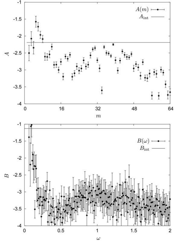
Fig. 12. Power-law exponents of the kinetic energy in Run V. top: A(|m|) , which are the exponents of cross-sectional energy spectra K_m(\omega) in Fig. 11, bottom: B(\omega) , which are the exponents of cross-sectional energy spectra K_\omega(|m|) in Fig. 11.
