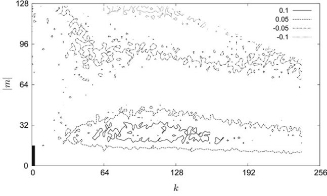
Fig. 8. Relative difference between energy spectra after about 1.5 days developed from the GM spectrum with and without energy in small horizontal wavenumbers E_d(k, |m|) .
