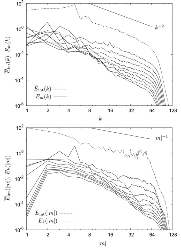
Fig. 5. Integrated and cross-sectional spectra of Run III. See the caption of Fig. 4 for details.
