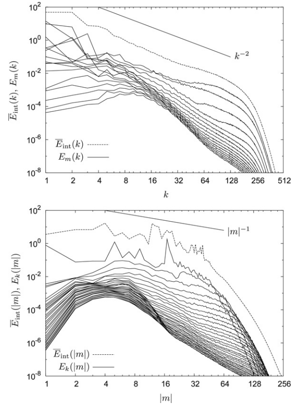
Fig. 10. Integrated and cross-sectional spectra of Run V. See the caption of Fig. 4 for details.
